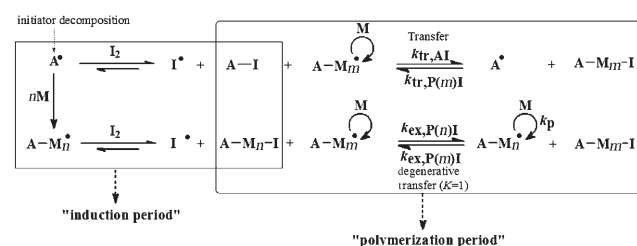
Scheme 1. Simplified mechanism of reverse iodine transfer polymerization (RITP) in solution (A•: radical from the initiator; I 2 : molecular iodine; M: monomer unit; n : mean number degree of polymerization).
