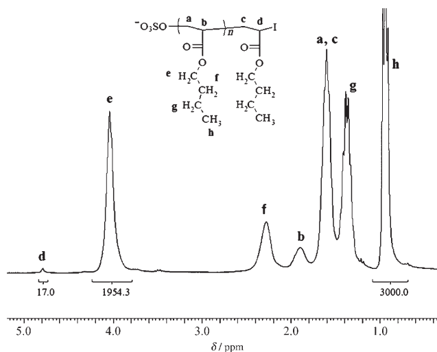
Figure 1. 1 H NMR spectrum in CDCl 3 of a PBUA–I latex synthesized by reverse iodine transfer polymerization (through ab initio emulsion polymerization) with NaI and coagulated in an aqueous CaCl 2 solution ([BuA]/[K 2 S 2 O 8 ]/[NaI] = 76.5:2.83:1, conversion of butyl acrylate: 74 %, M n,th = 7490 g mol -1 , M n,SEC = 7470 g mol -1 , polydispersity index: 1.84, M n,NMR = 7750 g mol -1 ): δ = 0.94 (t, H b ), 1.37 (m, H g ), 1.60 (m, H a , H c ), 1.90 (m, H b ), 2.28 (m, H f ), 4.04 (t, H e ), 4.79 ppm (m, H d ).
